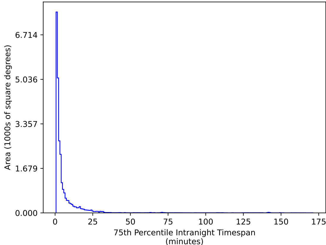
noroll_mjdp365_v3.4_10yrs All sky g band: 75th Percentile Intranight Timespan
