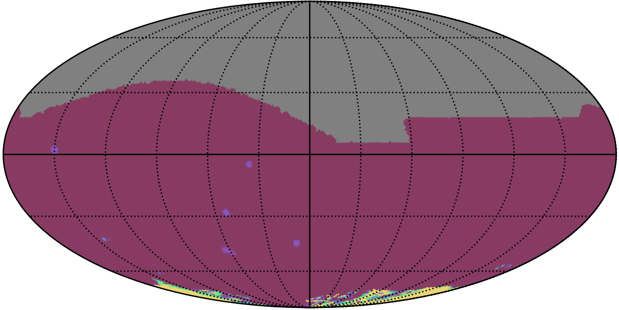
noroll_mjdp365_v3.4_10yrs All sky all bands: 75th Percentile Intranight Timespan
