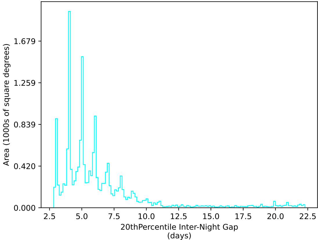
noroll_mjdp365_v3.4_10yrs WFD u band: 20thPercentile Inter-Night Gap
