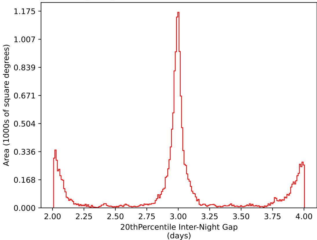
noroll_mjdp365_v3.4_10yrs WFD i band: 20thPercentile Inter-Night Gap
