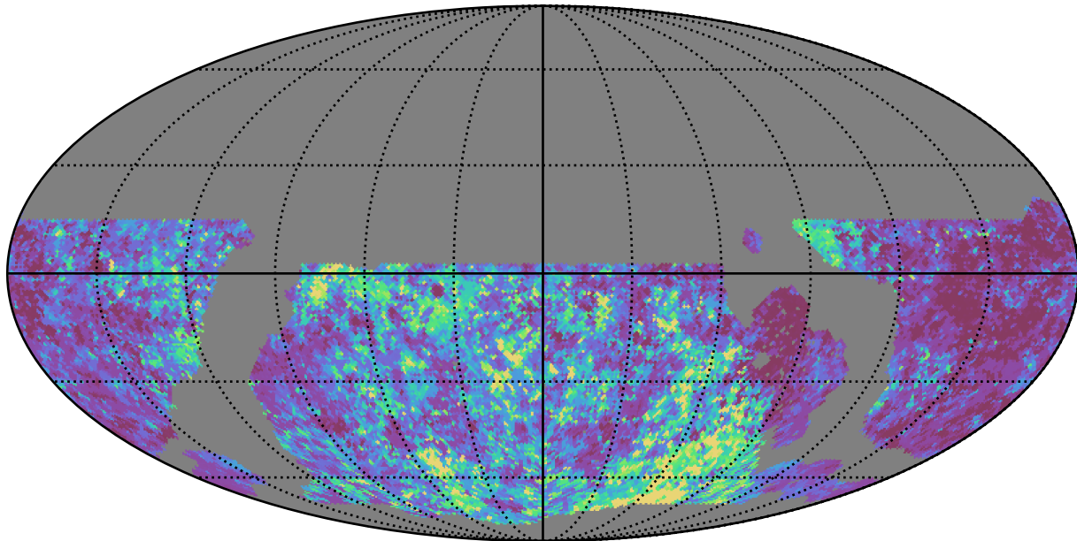
noroll_mjdp365_v3.4_10yrs WFD g band: 20thPercentile Inter-Night Gap
