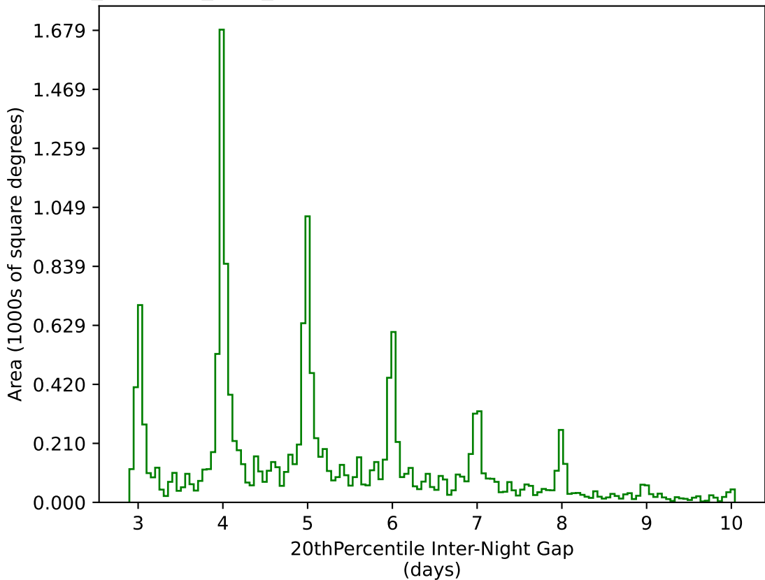
noroll_mjdp365_v3.4_10yrs WFD g band: 20thPercentile Inter-Night Gap
