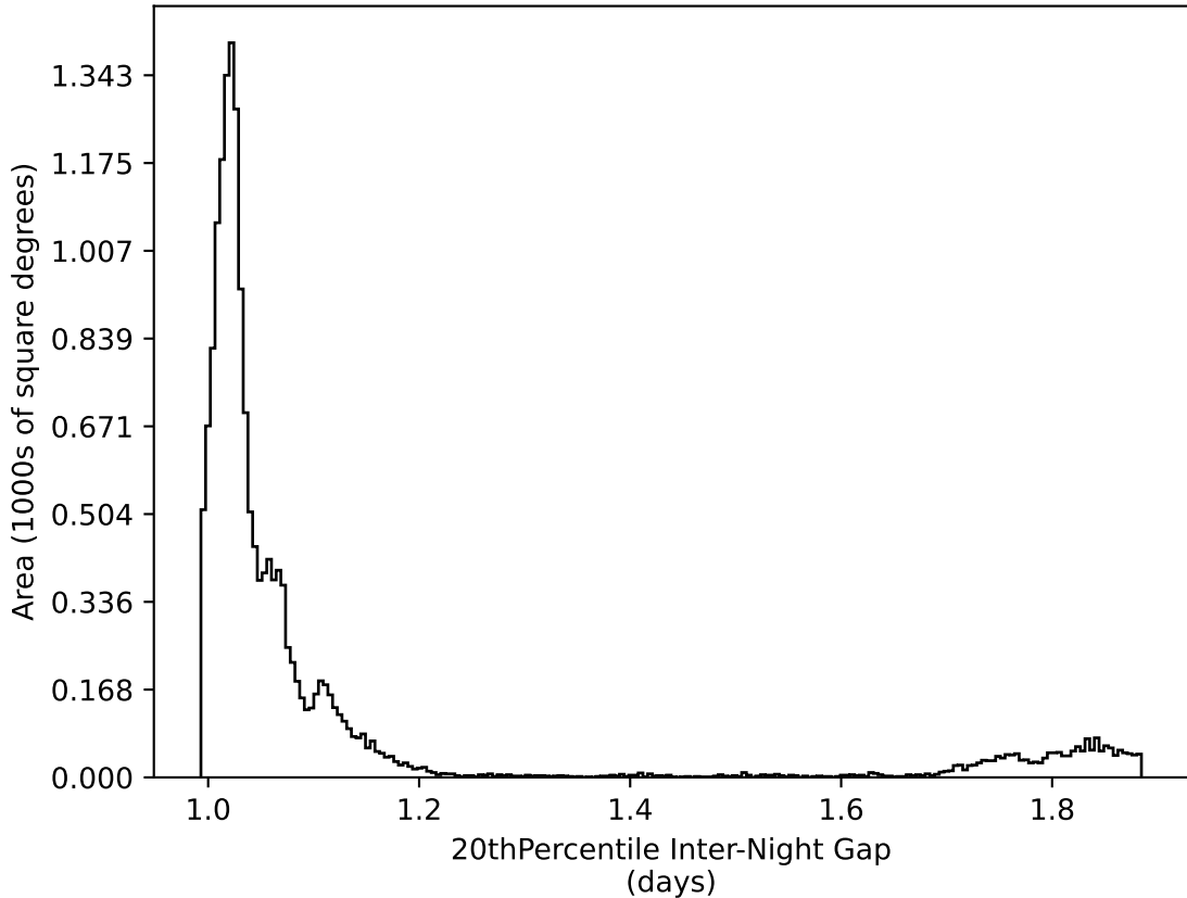
noroll_mjdp365_v3.4_10yrs WFD all bands: 20thPercentile Inter-Night Gap
