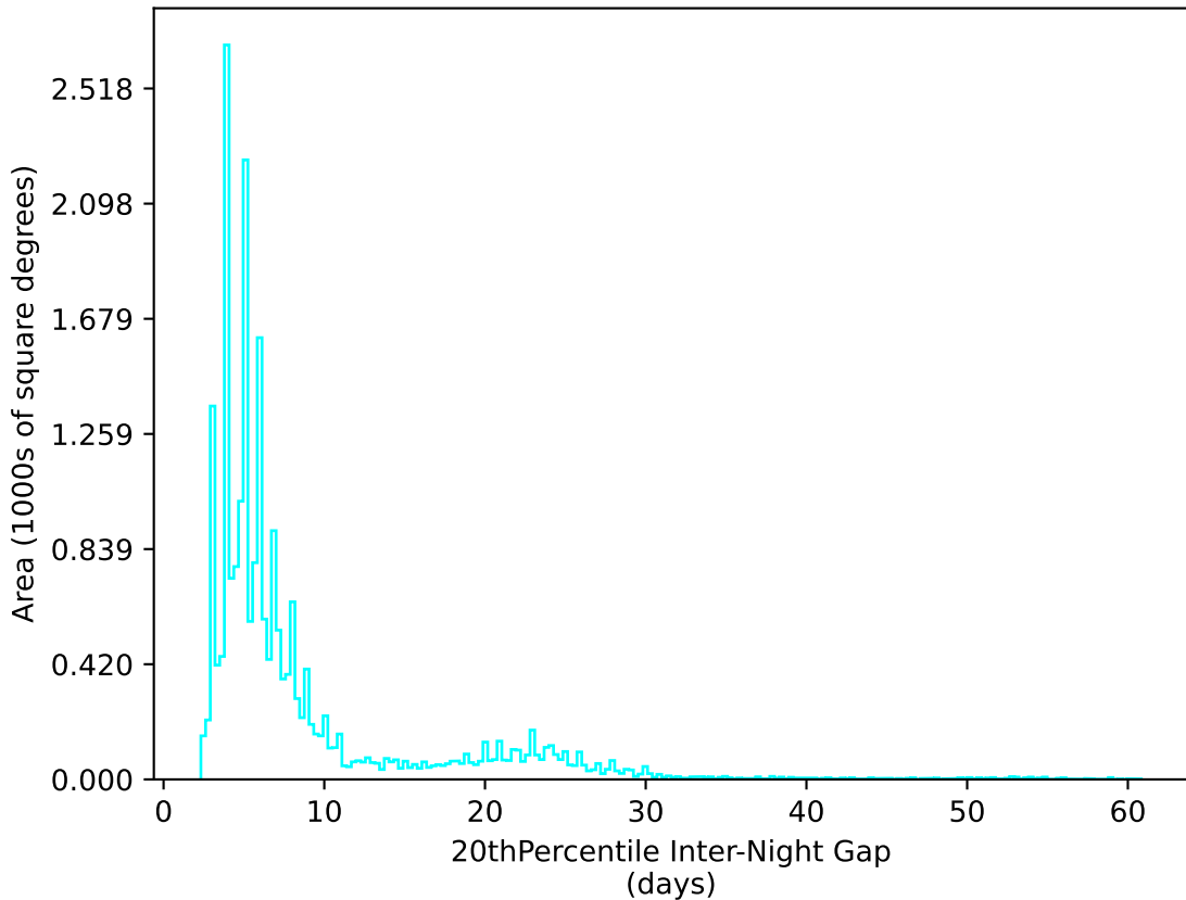
noroll_mjdp365_v3.4_10yrs All sky u band: 20thPercentile Inter-Night Gap
