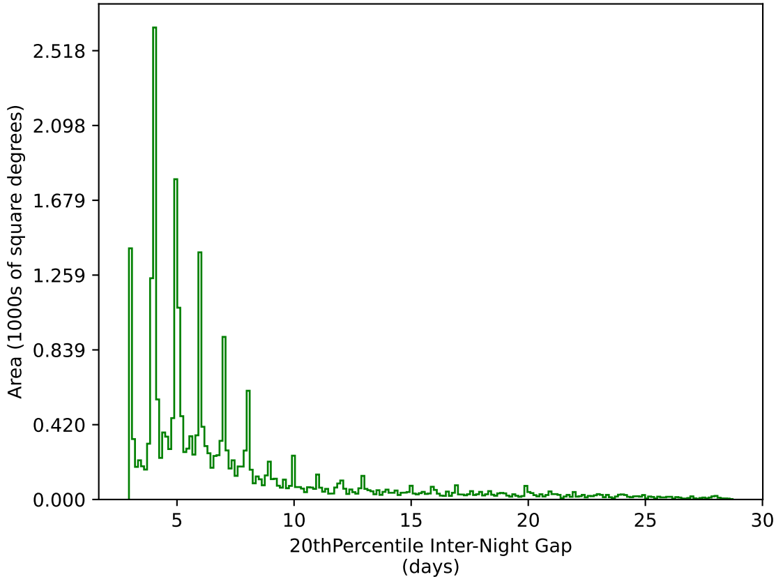
noroll_mjdp365_v3.4_10yrs All sky g band: 20thPercentile Inter-Night Gap
