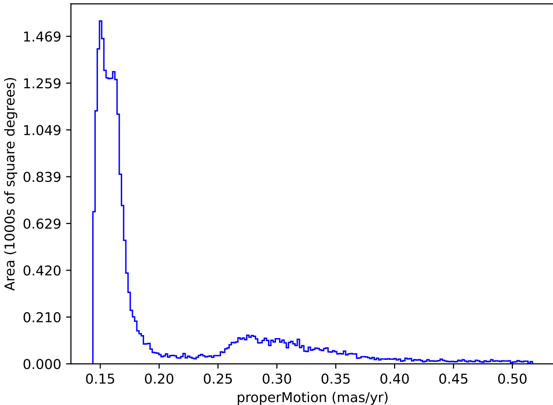
noroll_mjdp365_v3.4_10yrs : properMotion
