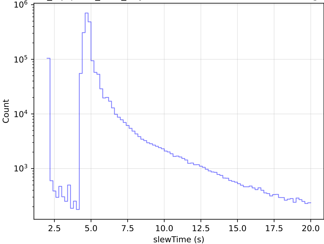
noroll_mjdp365_v3.4_10yrs All visits: Zoom Slew Time Histogram
