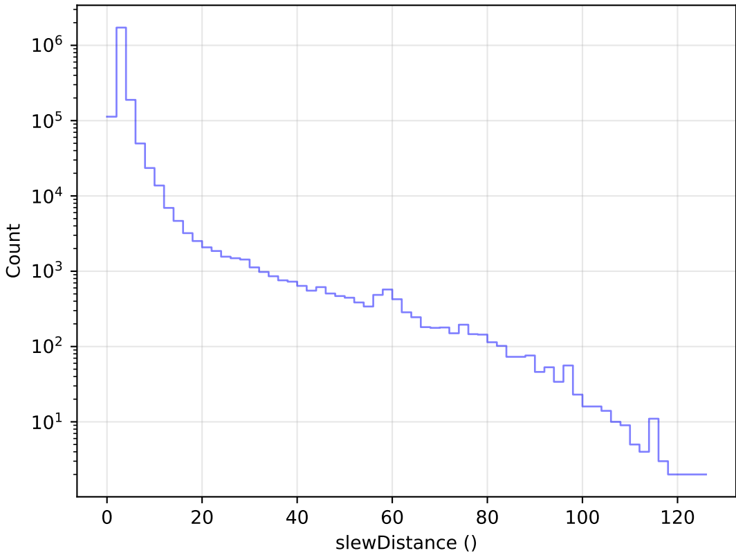
noroll_mjdp365_v3.4_10yrs All visits: Slew Distance Histogram
