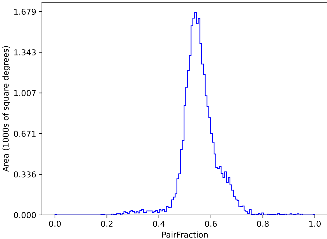
noroll_mjdp365_v3.4_10yrs (g or r or i): PairFraction
