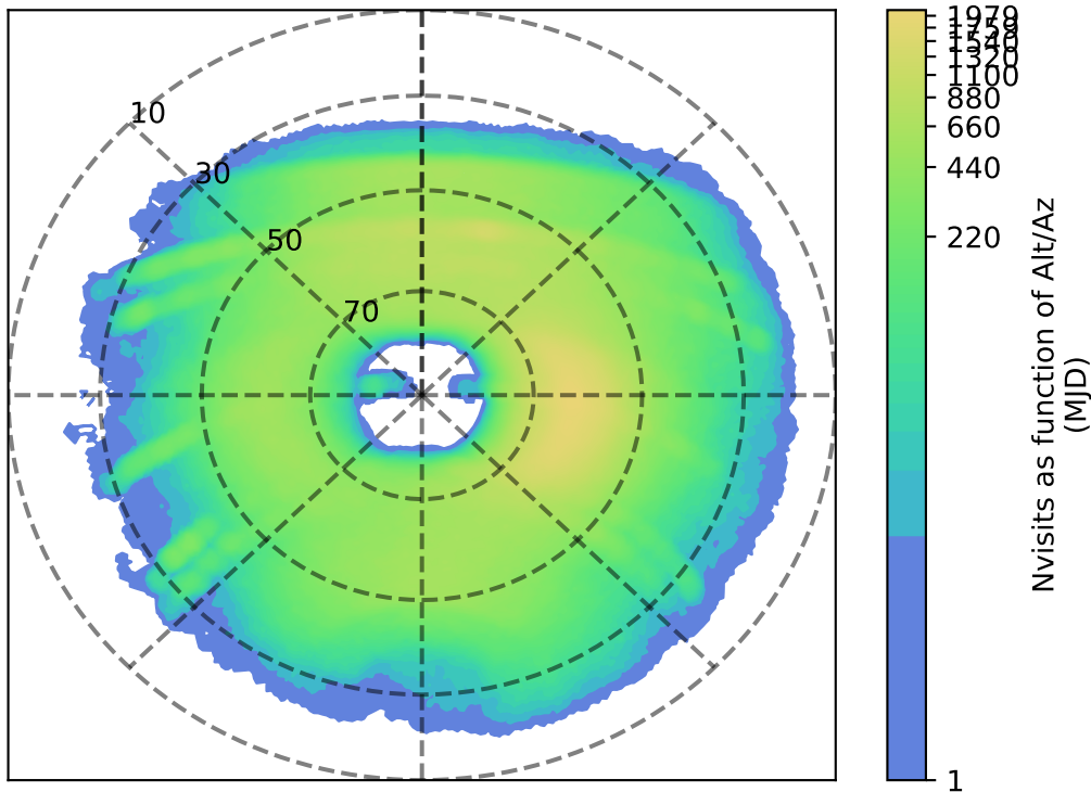
noroll_mjdp365_v3.4_10yrs y: Nvisits as function of Alt/Az
