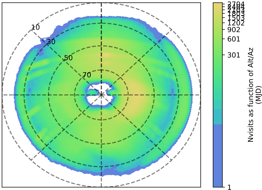
noroll_mjdp365_v3.4_10yrs i: Nvisits as function of Alt/Az
