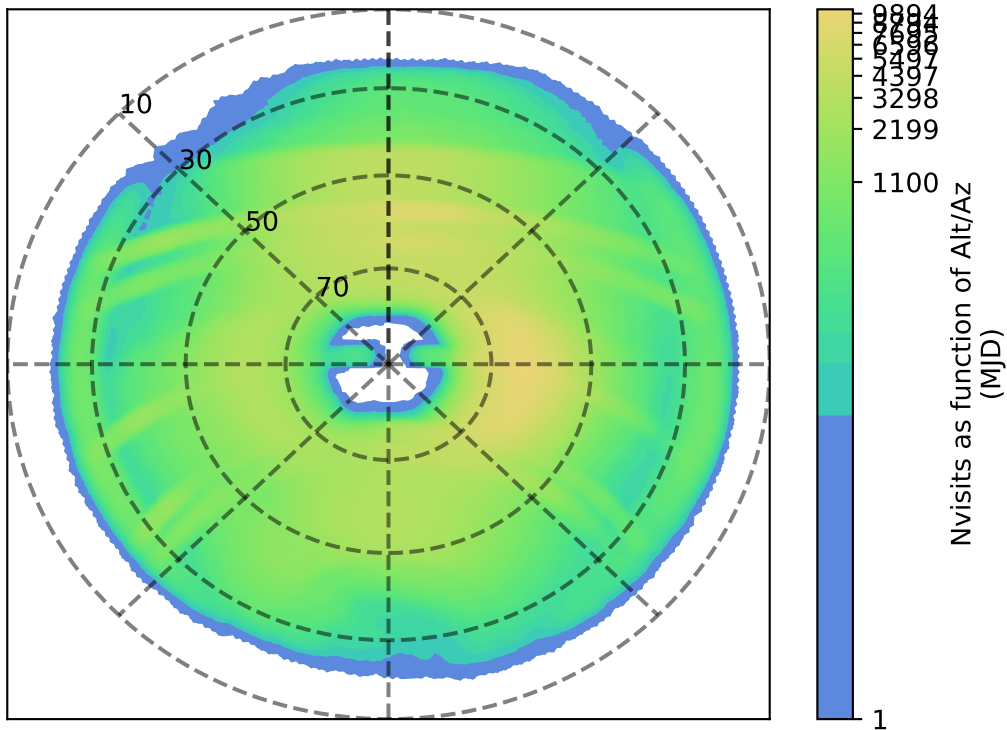
noroll_mjdp365_v3.4_10yrs : Nvisits as function of Alt/Az
