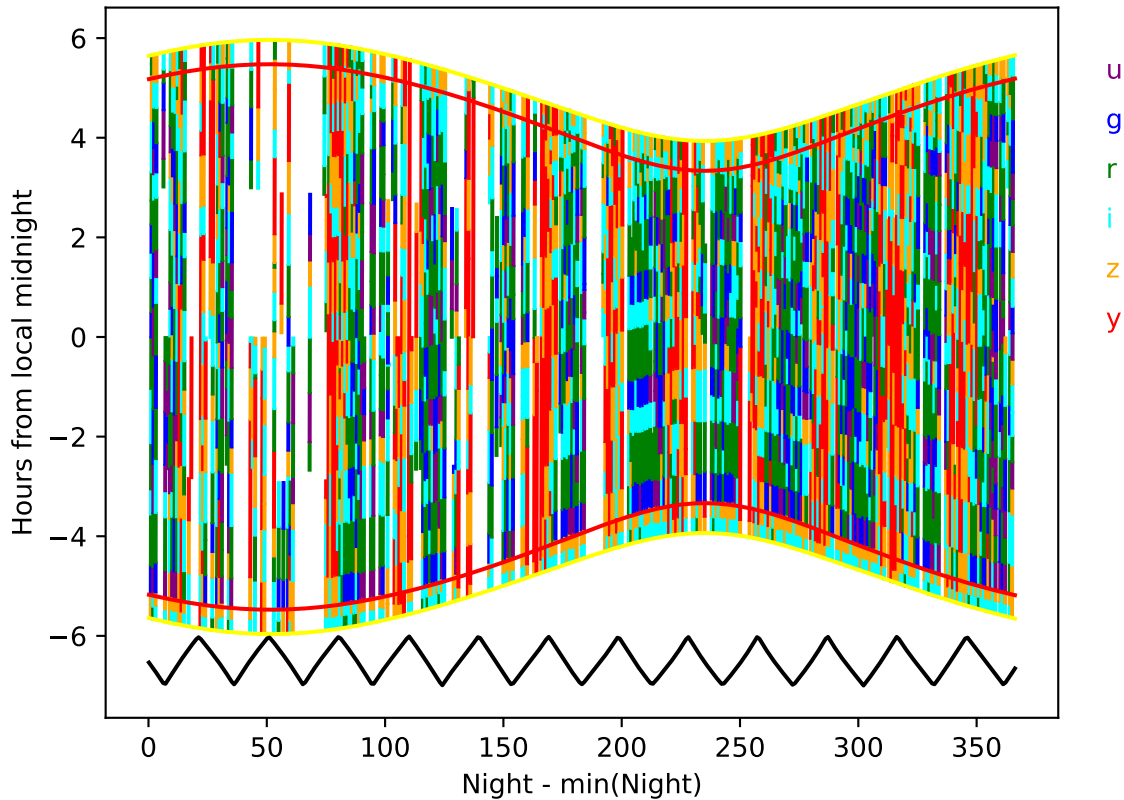
noroll_mjdp365_v3.4_10yrs year 9-10: Hourglass
