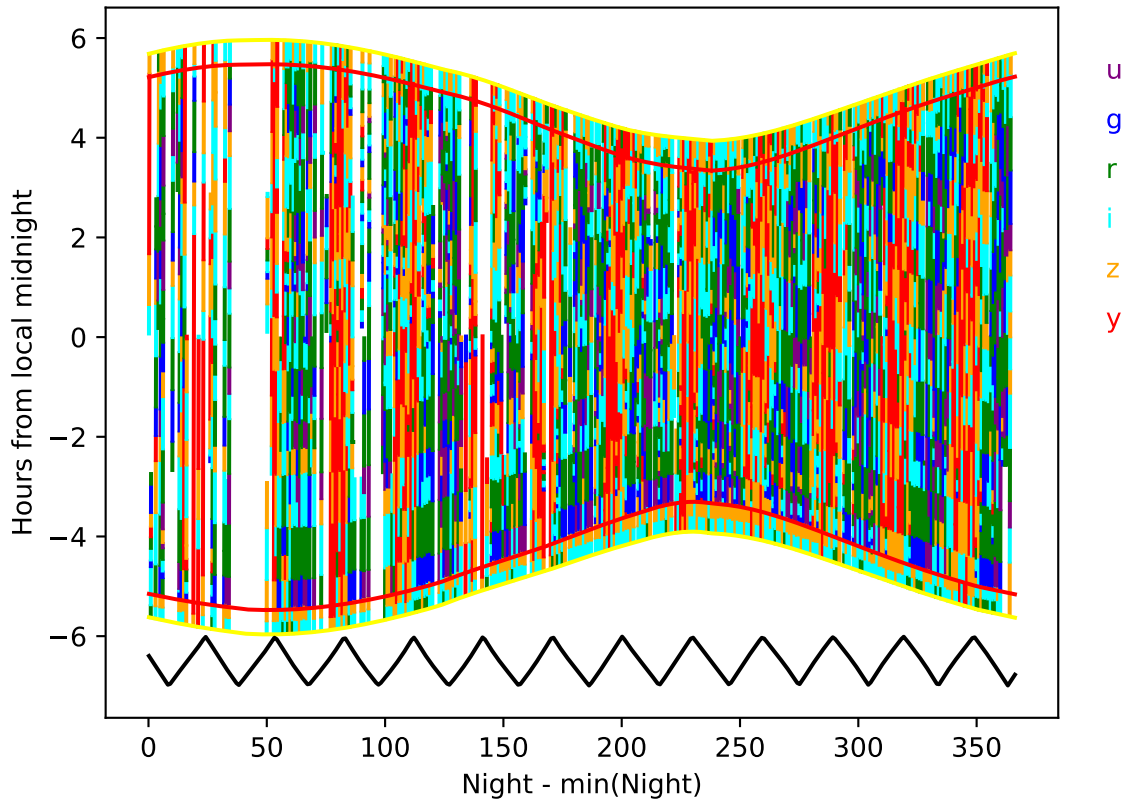
noroll_mjdp365_v3.4_10yrs year 6-7: Hourglass
