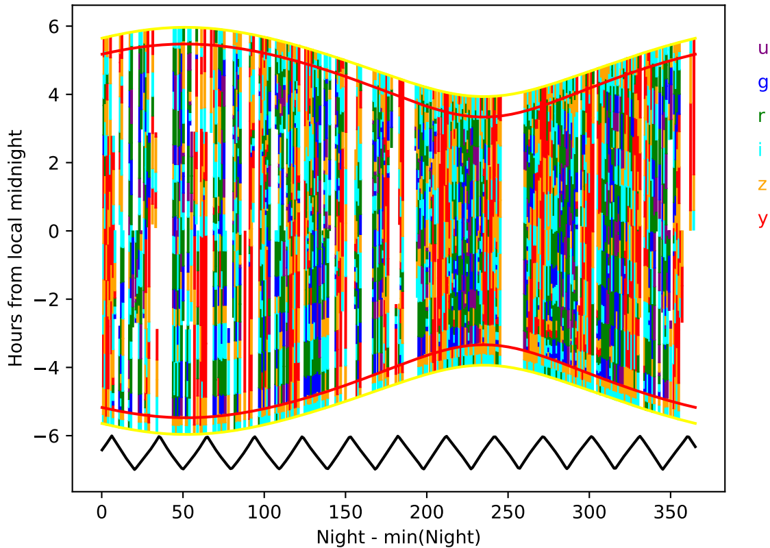
noroll_mjdp365_v3.4_10yrs year 5-6: Hourglass
