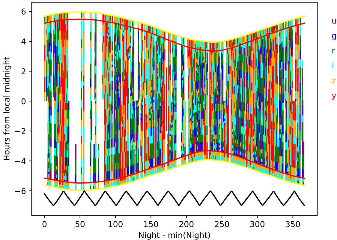
noroll_mjdp365_v3.4_10yrs year 3-4: Hourglass
