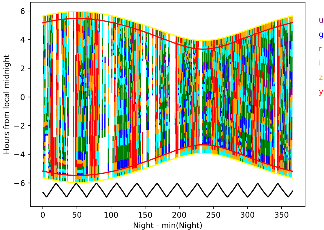
noroll_mjdp365_v3.4_10yrs year 1-2: Hourglass
