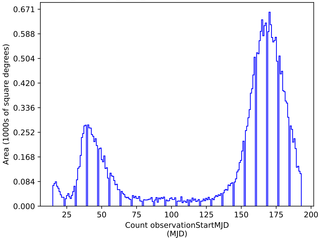
noroll_mjdp365_v3.4_10yrs z: Count observationStartMJD
