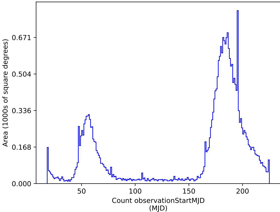
noroll_mjdp365_v3.4_10yrs r: Count observationStartMJD
