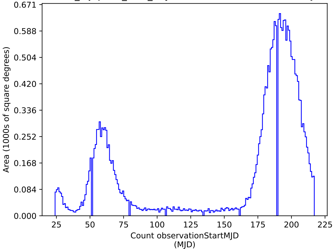
noroll_mjdp365_v3.4_10yrs i: Count observationStartMJD
