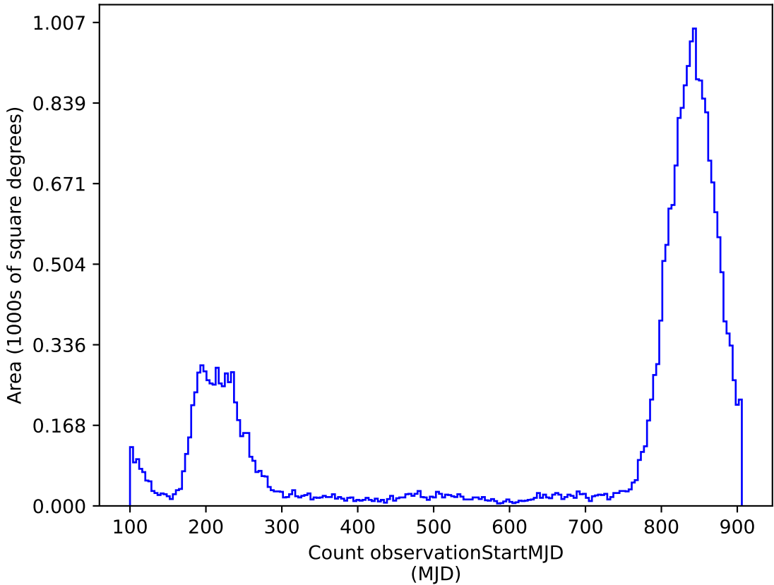
noroll_mjdp365_v3.4_10yrs : Count observationStartMJD
