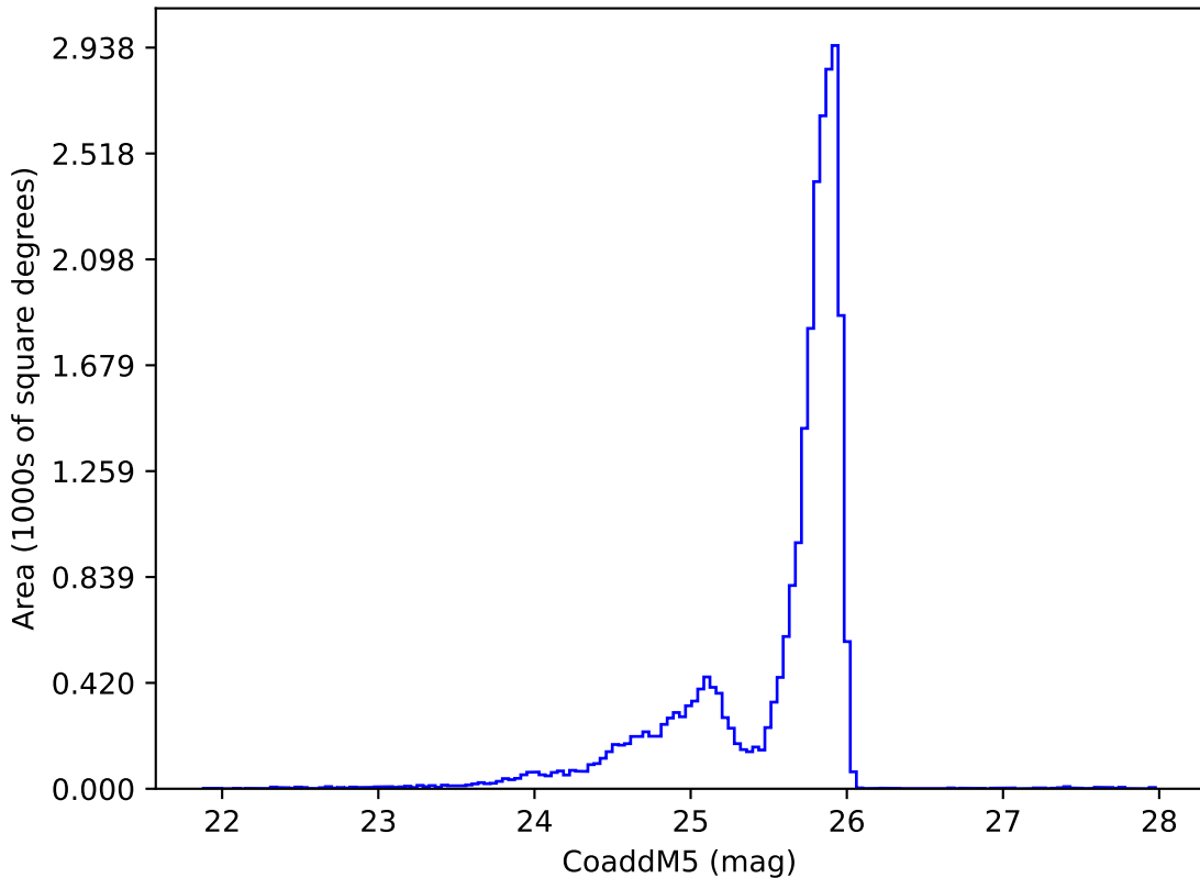
noroll_mjdp365_v3.4_10yrs z: CoaddM5
