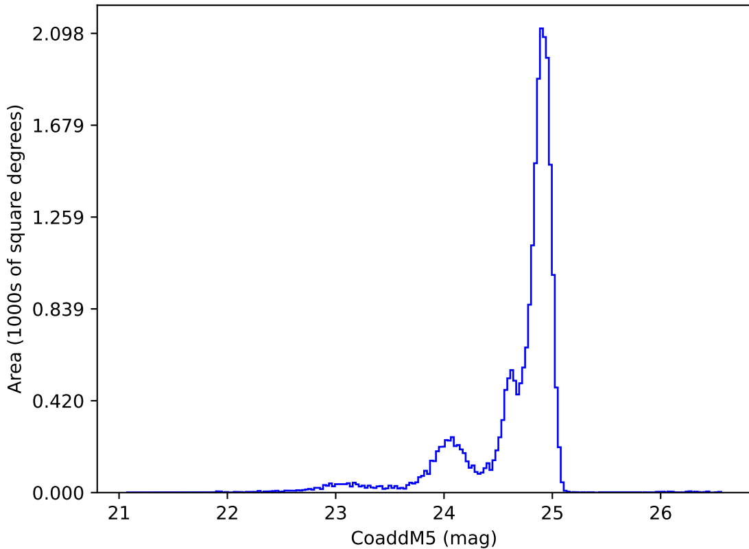
noroll_mjdp365_v3.4_10yrs y: CoaddM5
