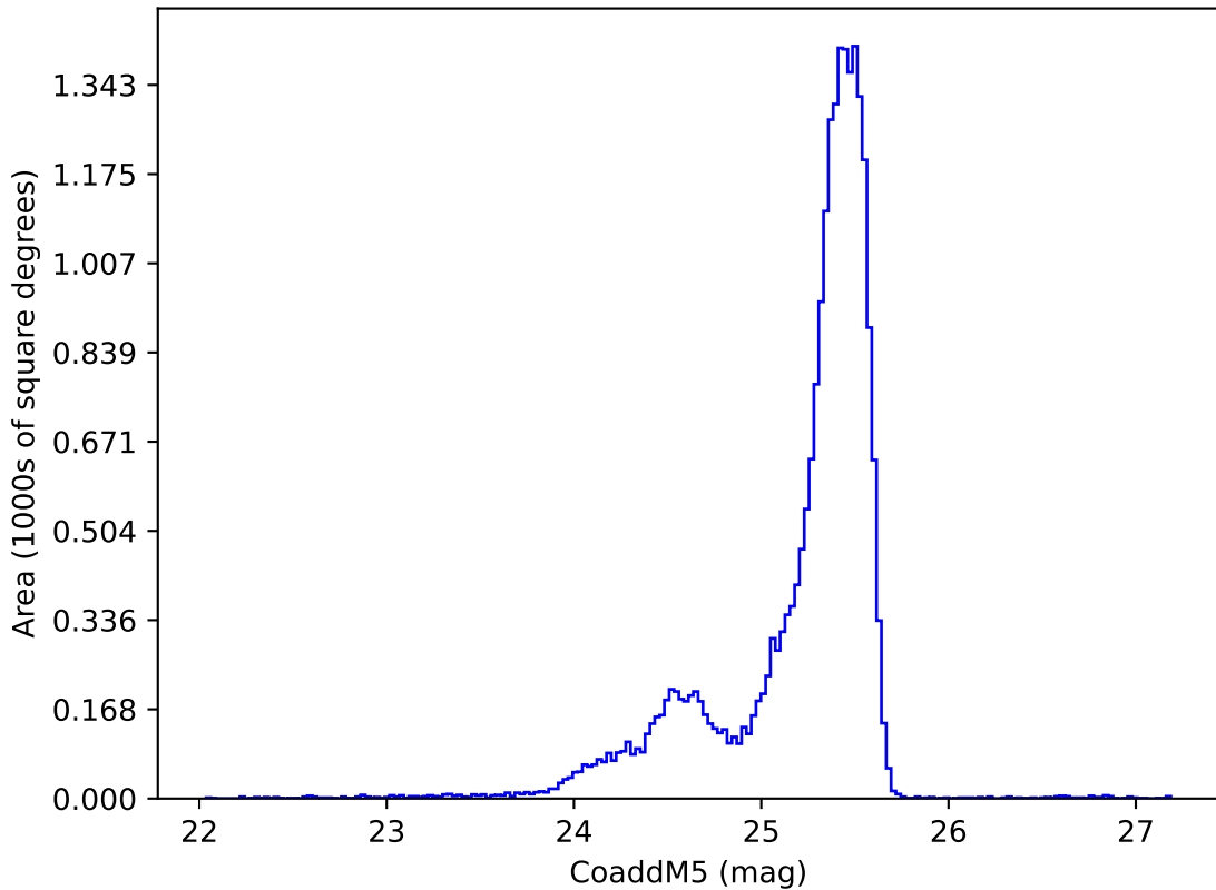
noroll_mjdp365_v3.4_10yrs u: CoaddM5
