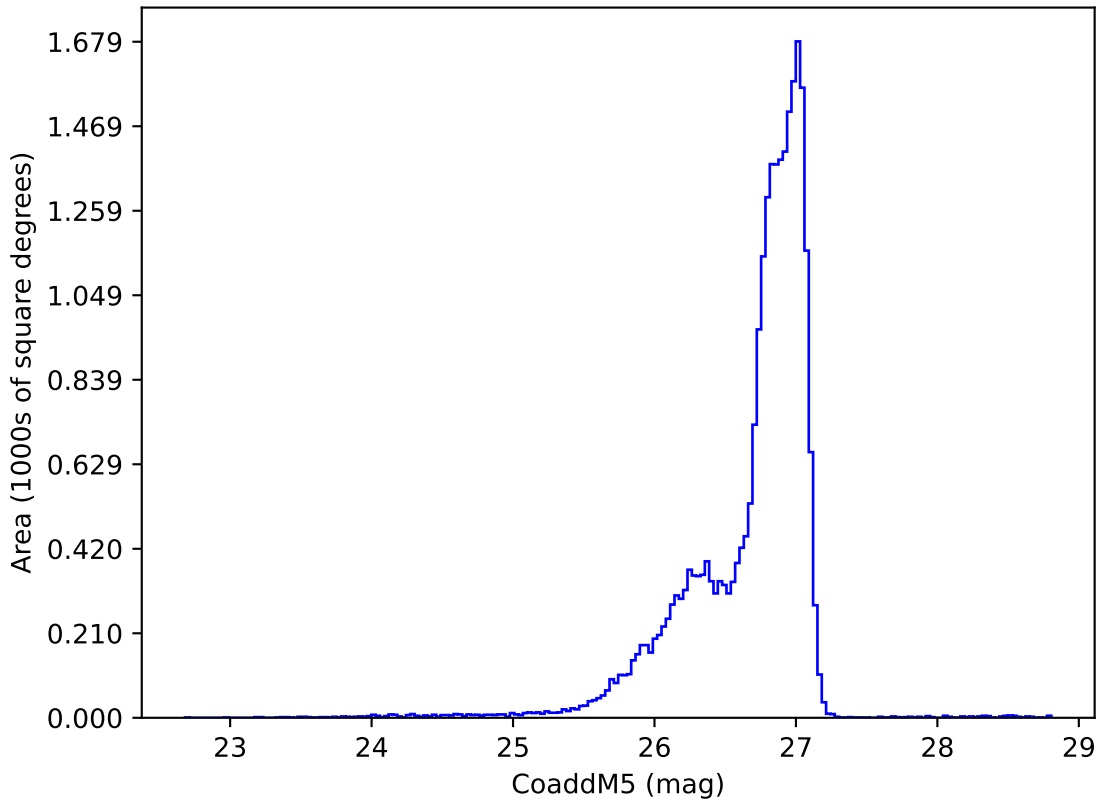
noroll_mjdp365_v3.4_10yrs g: CoaddM5
