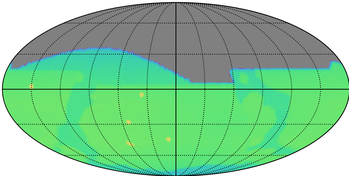
noroll_mjdp365_v3.4_10yrs : CoaddM5
