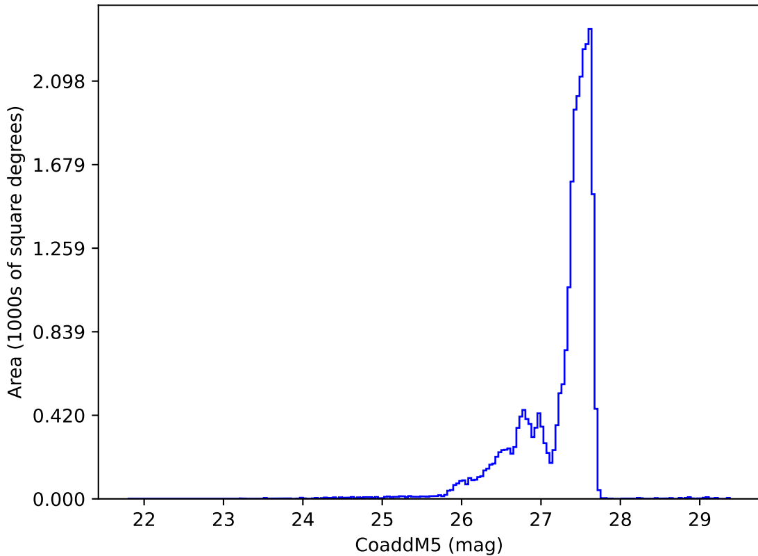
noroll_mjdp365_v3.4_10yrs : CoaddM5
