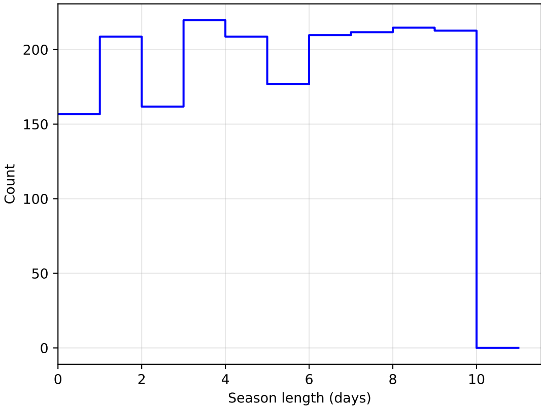
noroll_mjdp365_v3.4_10yrs DD:WFD all bands: SeasonLength
