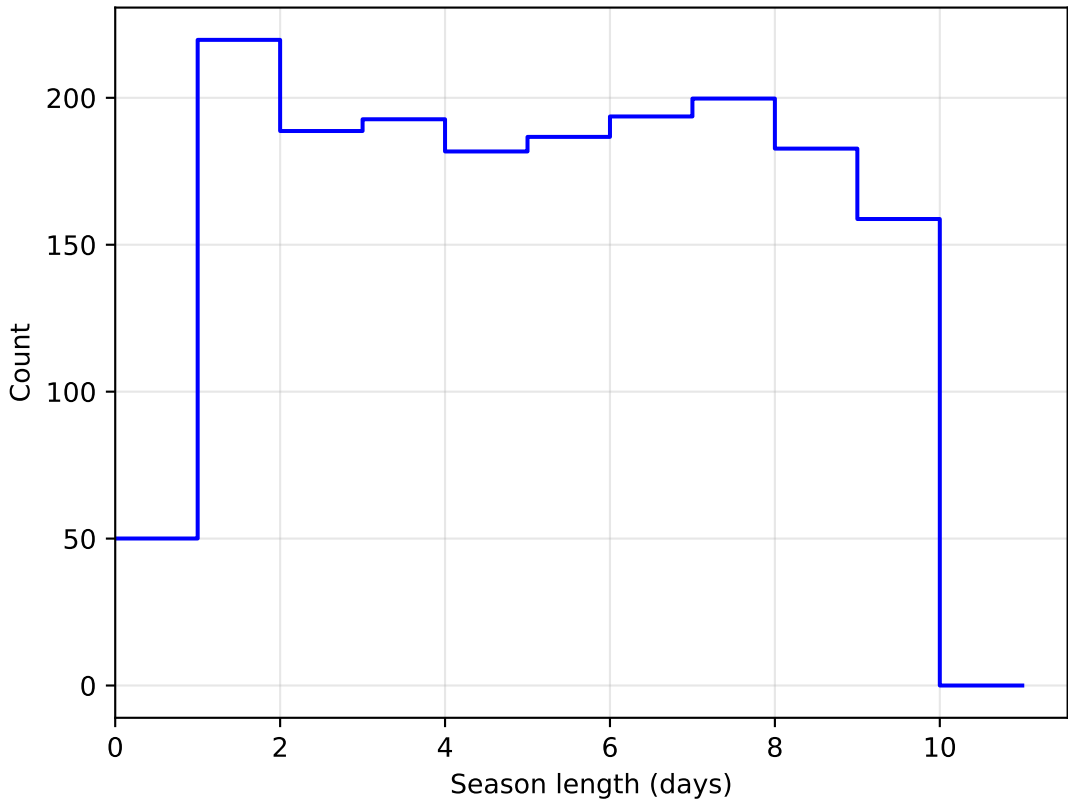
noroll_mjdp365_v3.4_10yrs DD: COSMOS all bands: SeasonLength
