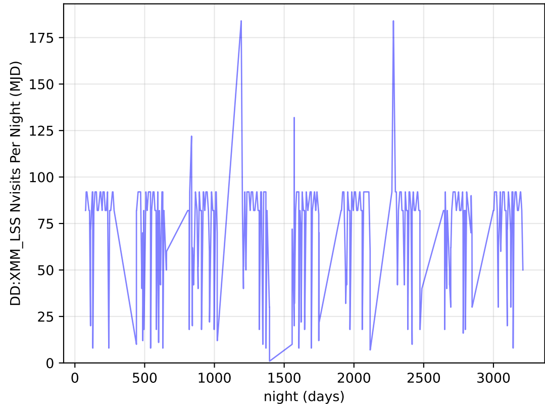
noroll_mjdp365_v3.4_10yrs all bands: DD:XMM_LSS Nvisits Per Night
