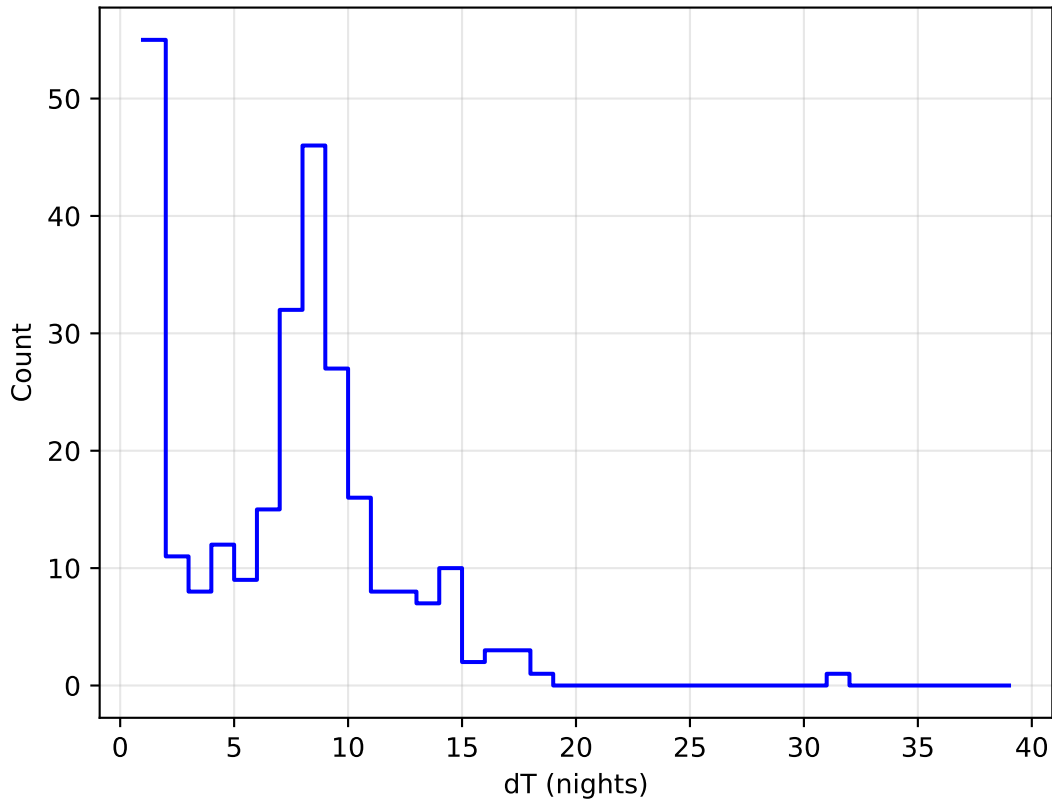
noroll_mjdp365_v3.4_10yrs all bands: DD:XMM_LSS Delta Nights Histogram
