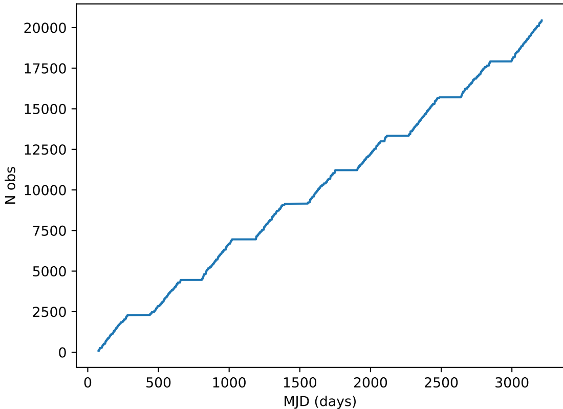
noroll_mjdp365_v3.4_10yrs all bands: DD:XMM_LSS Cumulative NVisits
