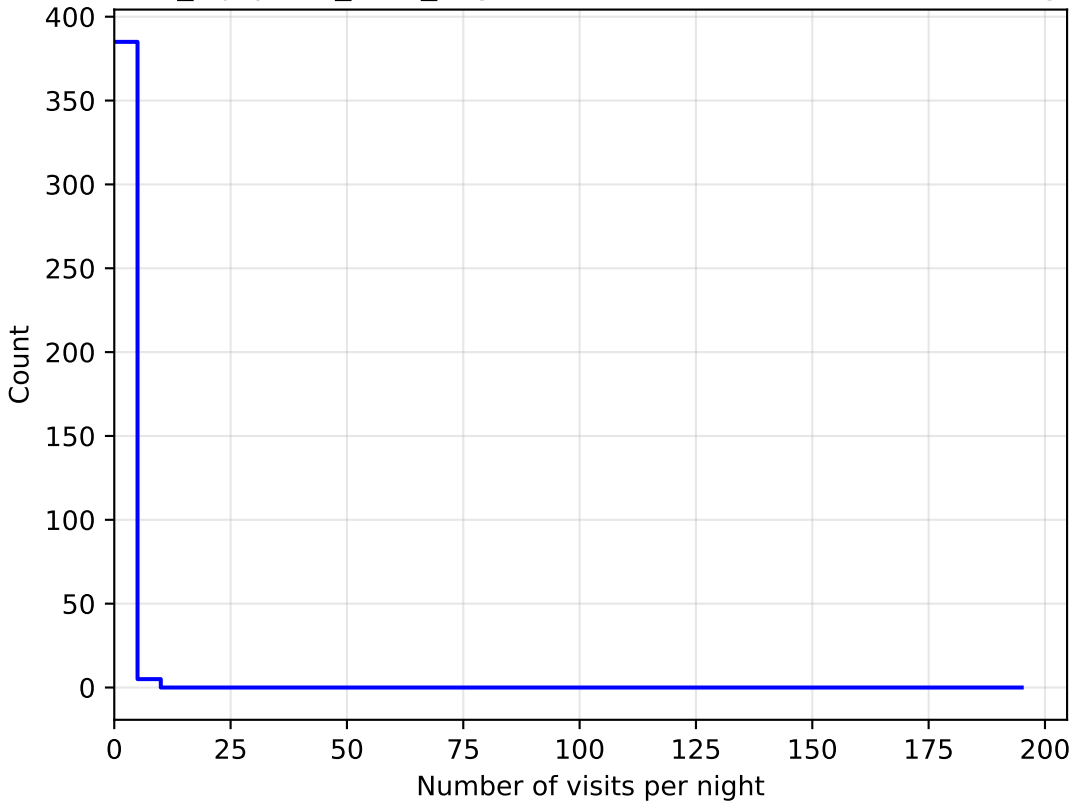
noroll_mjdp365_v3.4_10yrs all bands: DD:WFD NVisitsPerNight
