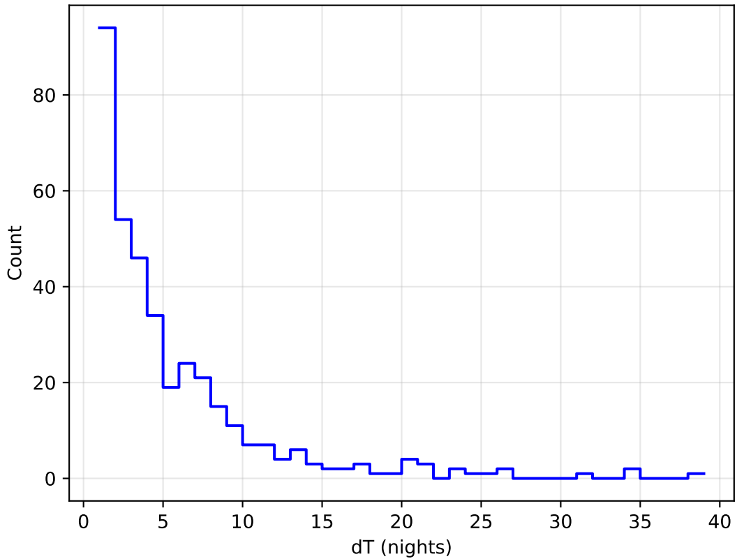
noroll_mjdp365_v3.4_10yrs all bands: DD:WFD Delta Nights Histogram
