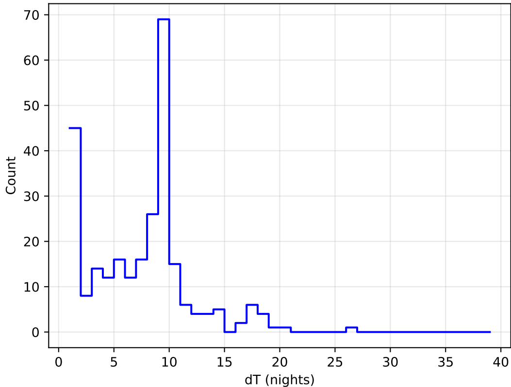
noroll_mjdp365_v3.4_10yrs all bands: DD:ELAISS1 Delta Nights Histogram
