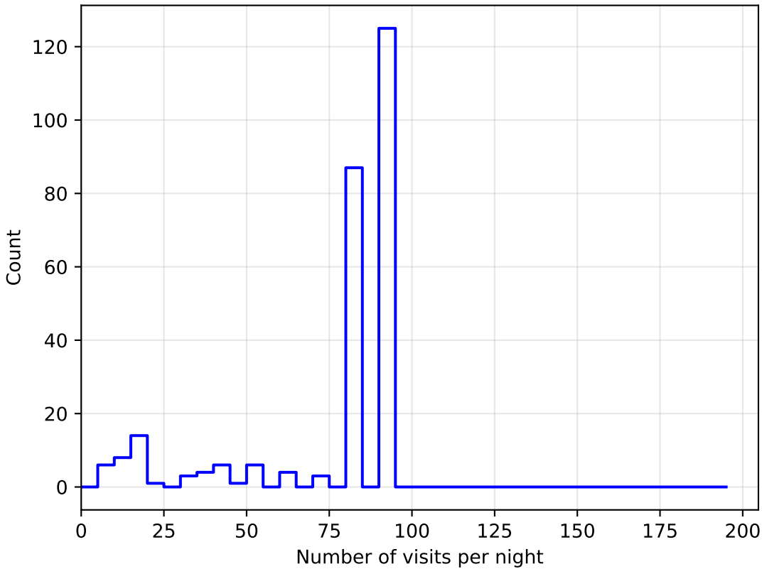
noroll_mjdp365_v3.4_10yrs all bands: DD:EDFS NVisitsPerNight
