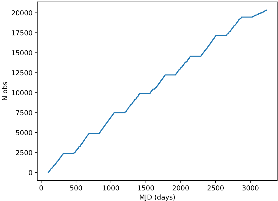
noroll_mjdp365_v3.4_10yrs all bands: DD:EDFS Cumulative NVisits
