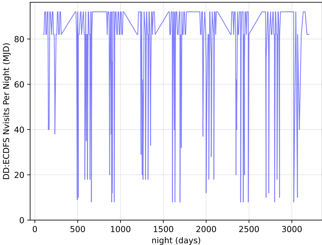
noroll_mjdp365_v3.4_10yrs all bands: DD:ECDFS Nvisits Per Night
