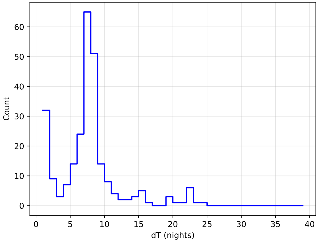
noroll_mjdp365_v3.4_10yrs all bands: DD:ECDFS Delta Nights Histogram
