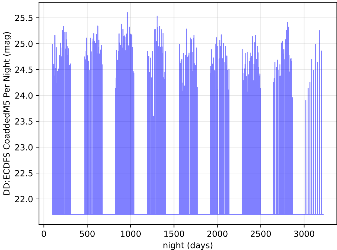
noroll_mjdp365_v3.4_10yrs z band: DD:ECDFS CoaddedM5 Per Night
