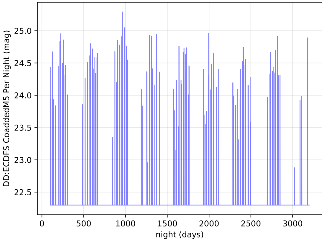
noroll_mjdp365_v3.4_10yrs u band: DD:ECDFS CoaddedM5 Per Night
