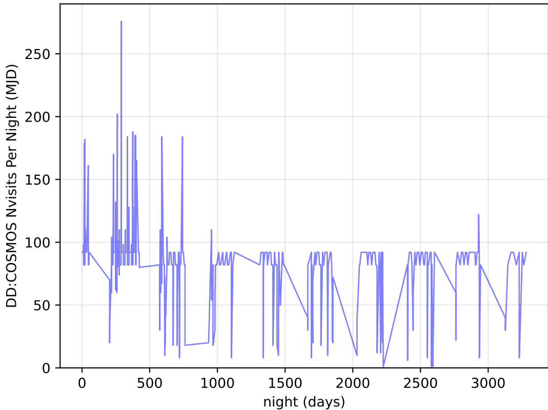
noroll_mjdp365_v3.4_10yrs all bands: DD:COSMOS Nvisits Per Night
