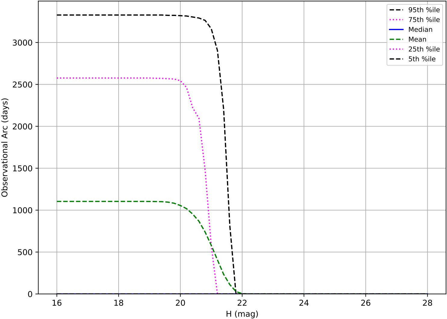
noroll_mjdp270_v3.4_10yrs: Observational Arc Length Vatira
