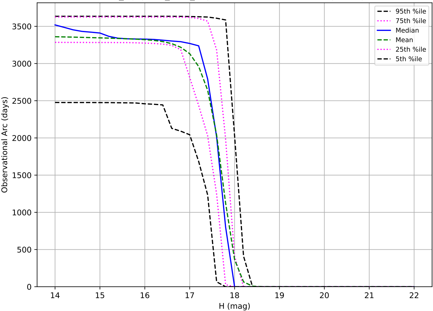
noroll_mjdp270_v3.4_10yrs: Observational Arc Length Trojan
