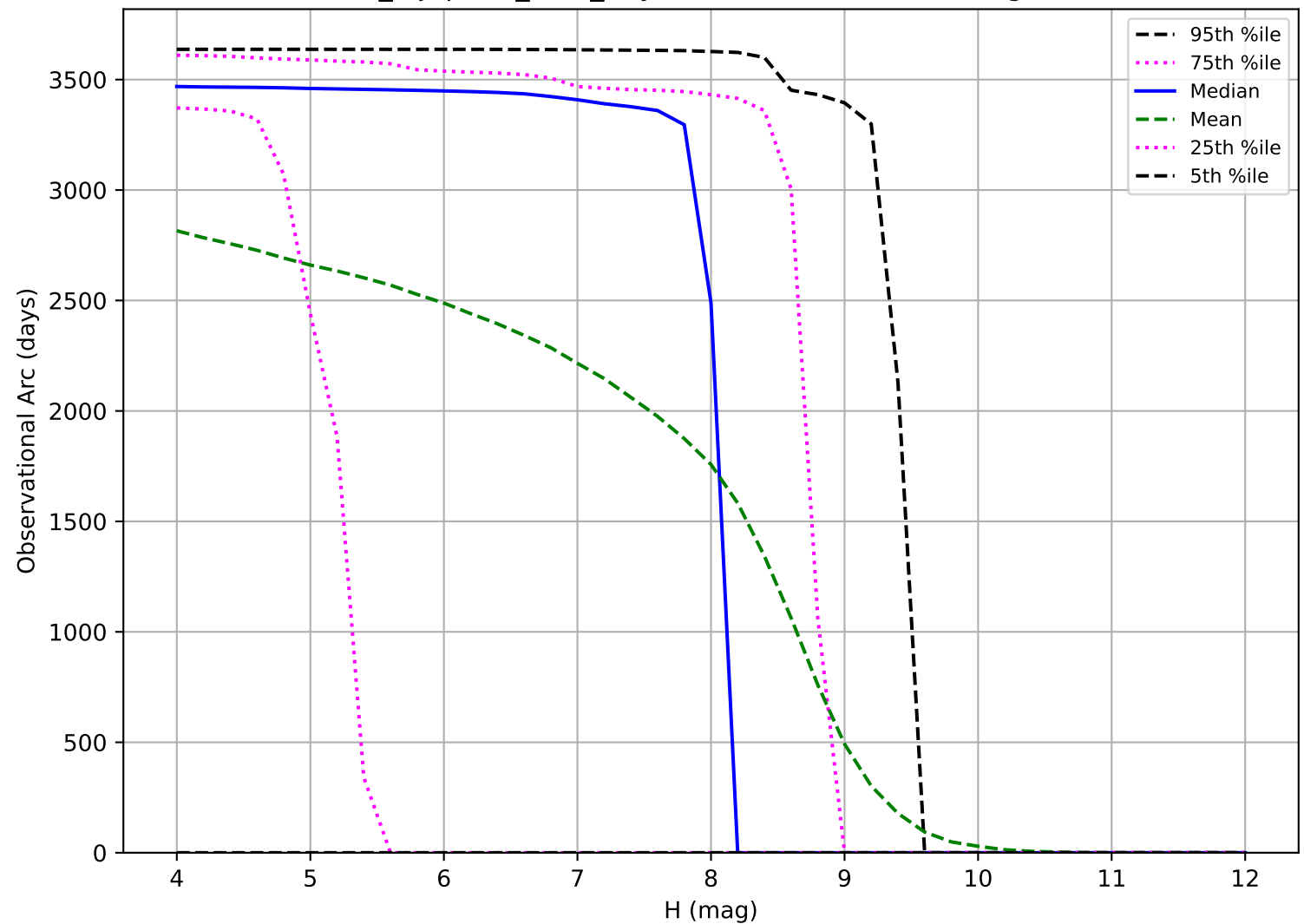
noroll_mjdp270_v3.4_10yrs: Observational Arc Length TNO
