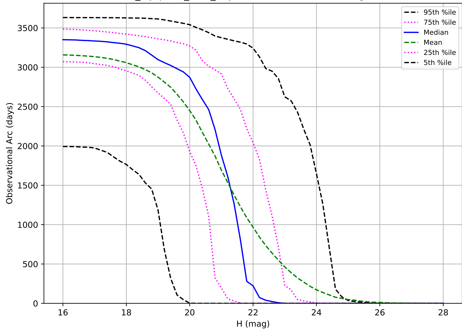
noroll_mjdp270_v3.4_10yrs: Observational Arc Length PHA
